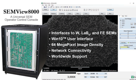
SEMView8000 Operator Control Console with Win10 User Interface Software
